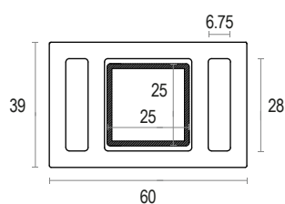
Frangisole Slim in Wpc
