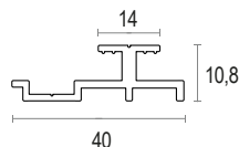
Clip in alluminio AF610
