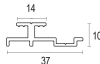
Clip in alluminio AF609
